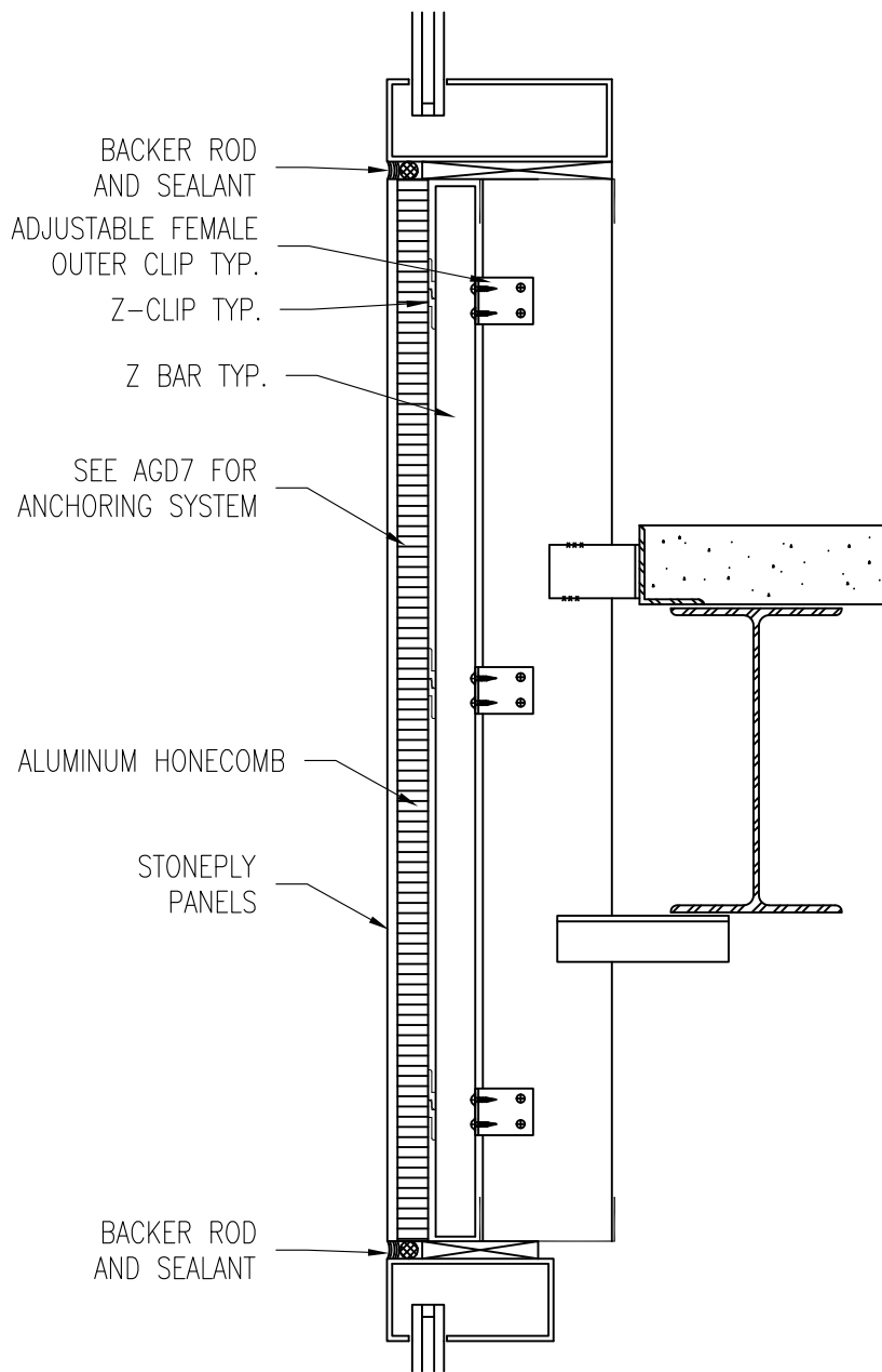
FC3A SPANDREL FIELD CONDITION
